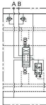
Electrohydraulic actuation
