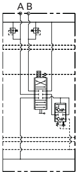
Mechanical lever actuation
