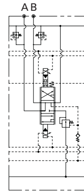
Electrohydraulic actuation
