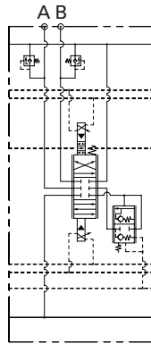
Electrohydraulic actuation
