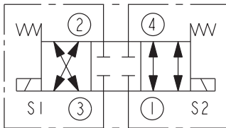
HSV10-47C High Pressure Spool 4-Port, 3-Position, Closed Center
