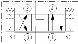
HSP10-47D High Pressure Spool 4-Port, 3-Position, Closed Center
