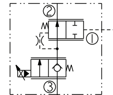
HSPECxx-34 Relief, Directing Acting Poppet with Reverse Flow Check
