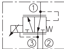
EHPR98-G3x Proportional, Reducing / Relieving, Drop-in
