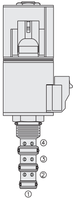
HSP10-47D High Pressure Spool 4-Port, 3-Position, Closed Center
