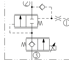
HSPECxx-30 Proportional Flow Control Valve with Integral Compensator
