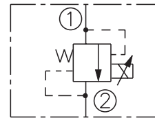
TSxx-27 Proportional Pressure Control, Pilot-Operated Relief
